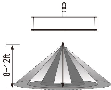
Height of installation 8~12ft
